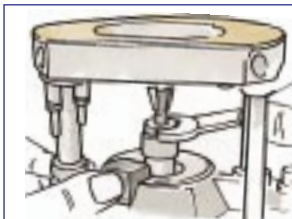
On some routers a spindle lock allows the collet nut to be tightened with only one spanner.
