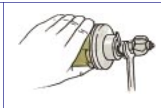
On other types a tommy bar is fitted through the spindle and a spanner used to tighten the collet nut
